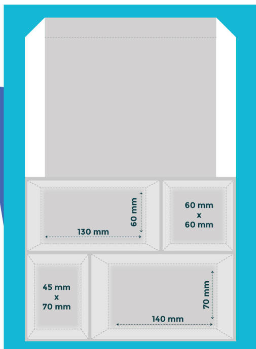
Lunch Box 4 Compartment (190 x 155 x 50 mm)
